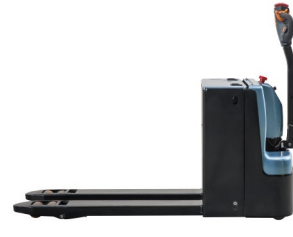
P20/25 Capacity: 2.0/2.5T Fork Width: 540/685mm Fork Length: 1150/1220mm ZAPI Full AC Battery: 24V 240/270AH
